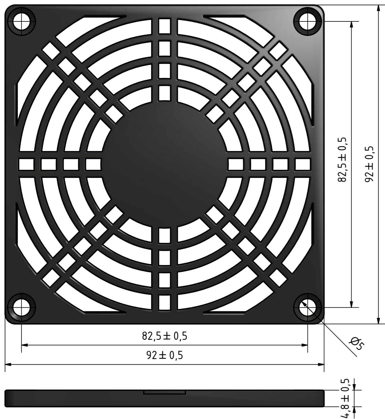
Innengitter
